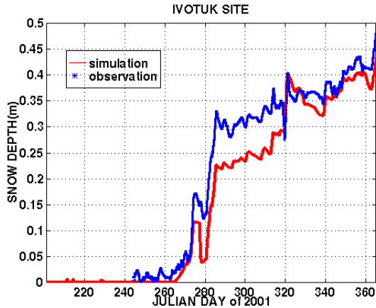
Figure 6. Simulated and observed snow cover for Julian days 201-365, 2001 at the Ivotuk Moss site.
