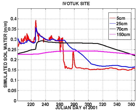
Figure 7. Simulated liquid soil moisture for Julian days 201-365, 2001 at the Ivotuk Moss site
