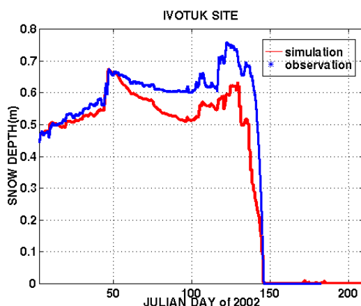
Figure 1. Simulated and observed snow cover for Julian days 3-209 of 2002 at the Ivotuk Moss site.
