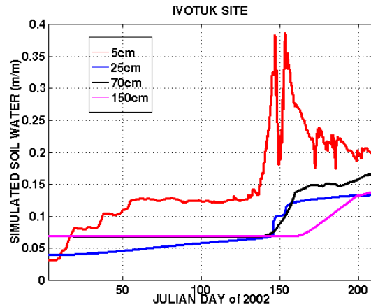
Figure 4. Simulated liquid soil moisture for Julian days 3-209 of 2002 at the Ivotuk Moss site.
