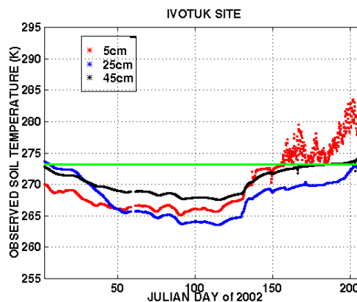
Figure 3. Observed soil temperatures for Julian days 3-209 of 2002 at the Ivotuk Moss site.
