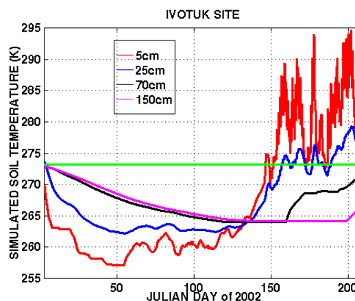
Figure 2. Simulated soil temperatures for Julian days 3-209, 2002 at the Ivotuk Moss site.
