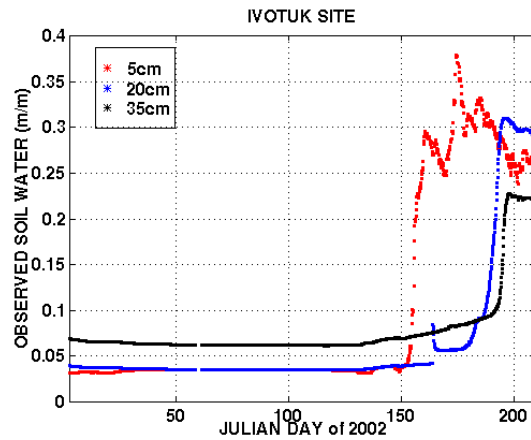
Figure 5. Observed liquid soil moisture for Julian days 3-209 of 2002 at the Ivotuk Moss site.
