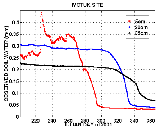
Figure 8. Observed liquid soil moisture for Julian days 201-365, 2001 at the Ivotuk Moss site
